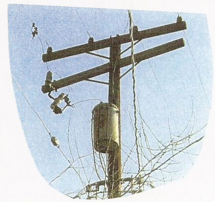
Photo 6 4 failed insulator pins 2486 E. Fisher Lane
