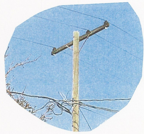
(Photo 12) North side of 2940 S. 2300 E. 2 Failed insulator pins
