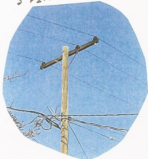
Photo 9 Multiple Outages 3 Failed insulators
