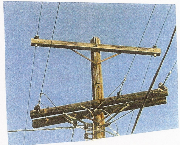
(Photo 12) North side of 2940 S. 2300 E. 2 Failed insulator pins
