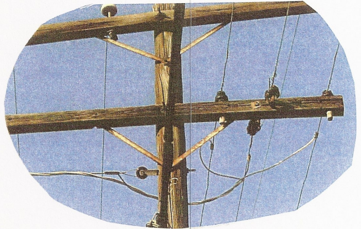
Photo 22 2036 E. Lambourn 1 Failed insulator pin
