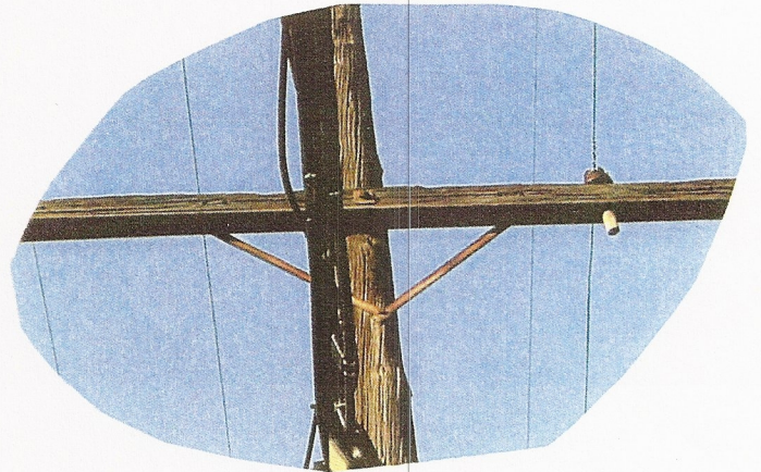
Photo 22 2036 E. Lambourn 1 Failed insulator pin
