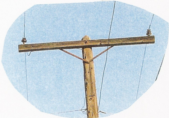
Photo 21 End of Aveline Ave that runs off Connor st. (West 3127 Aveline) 1 Failed insulator pins
