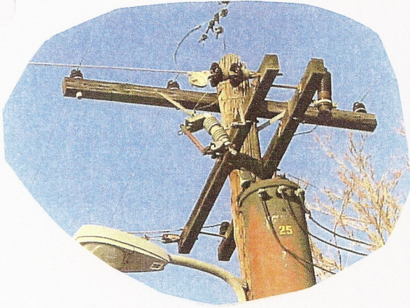
Photo 21 End of Aveline Ave that runs off Connor st. (West 3127 Aveline) 1 Failed insulator pins
