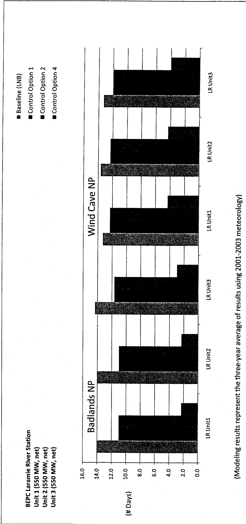
Figure 8 – Modeled BART Impacts: Number of Days > 0.5 delta-dv
