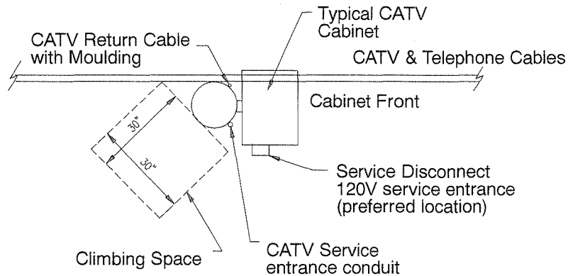
Figure 3 - Climbing Space
