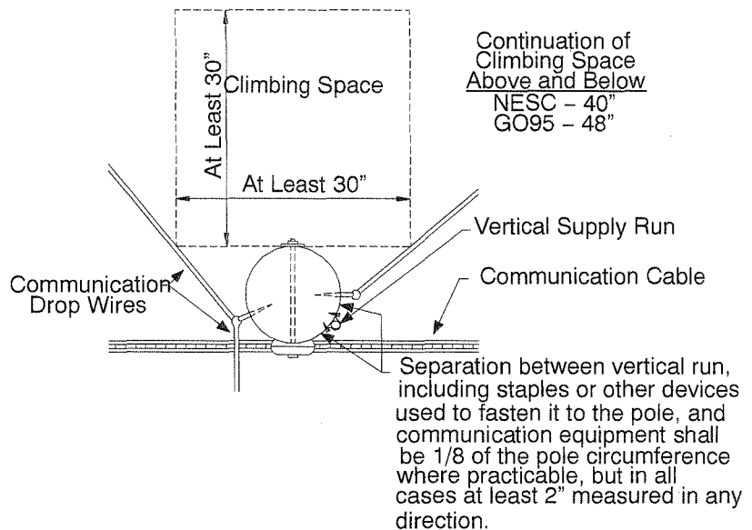
Figure 5—Climbing Space
