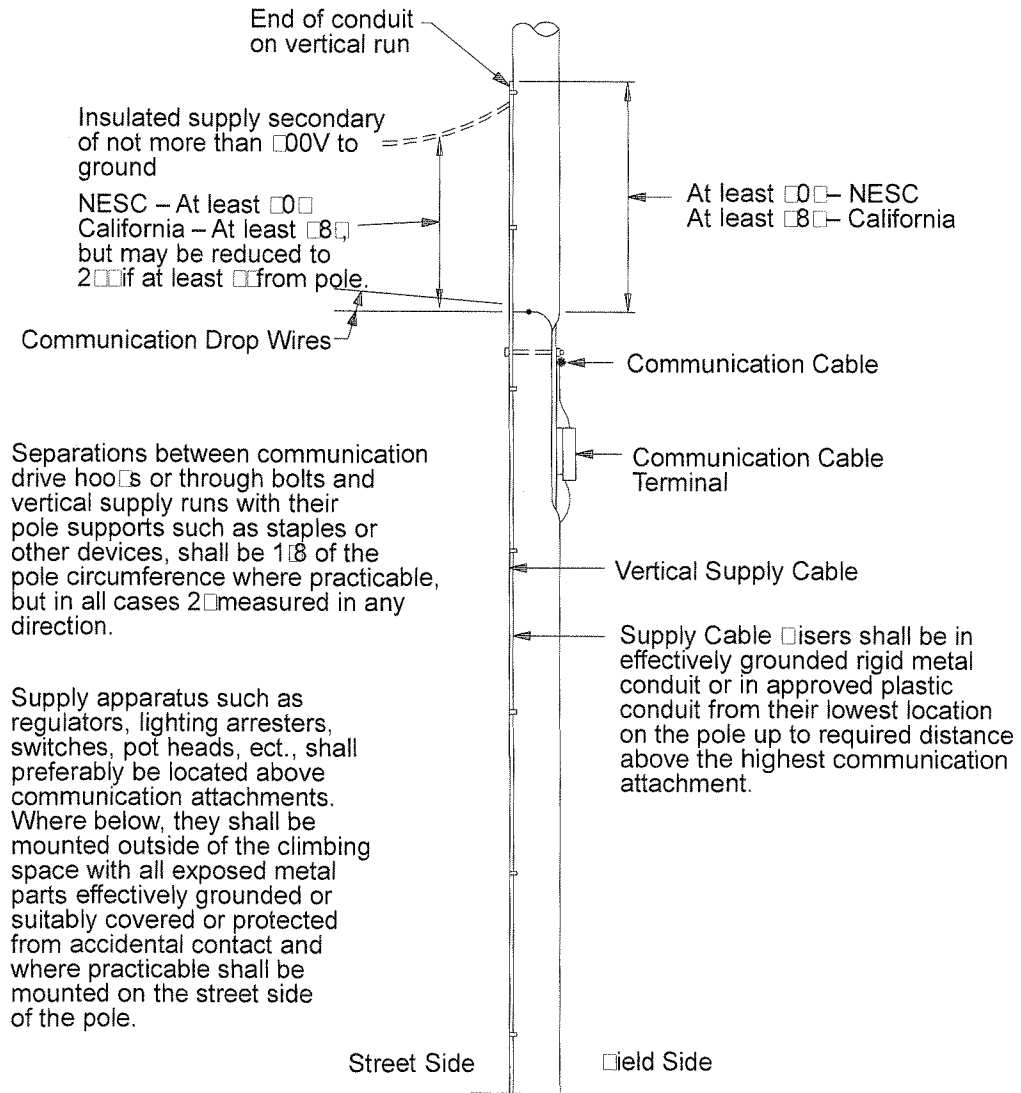
Figure 1 - Supply Riser on Joint Use Pole
