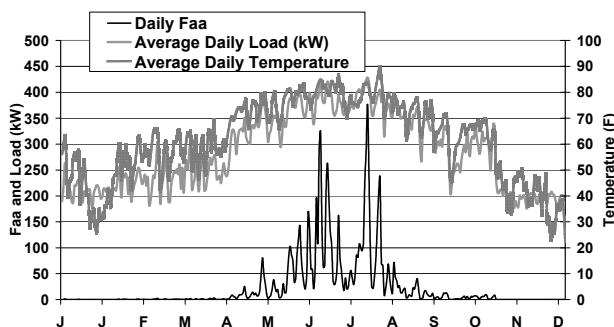
Figure 4 – Daily aging hours for Atlanta nursing home load
