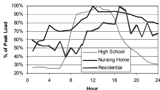
Figure 2 – Peak day load profiles.
