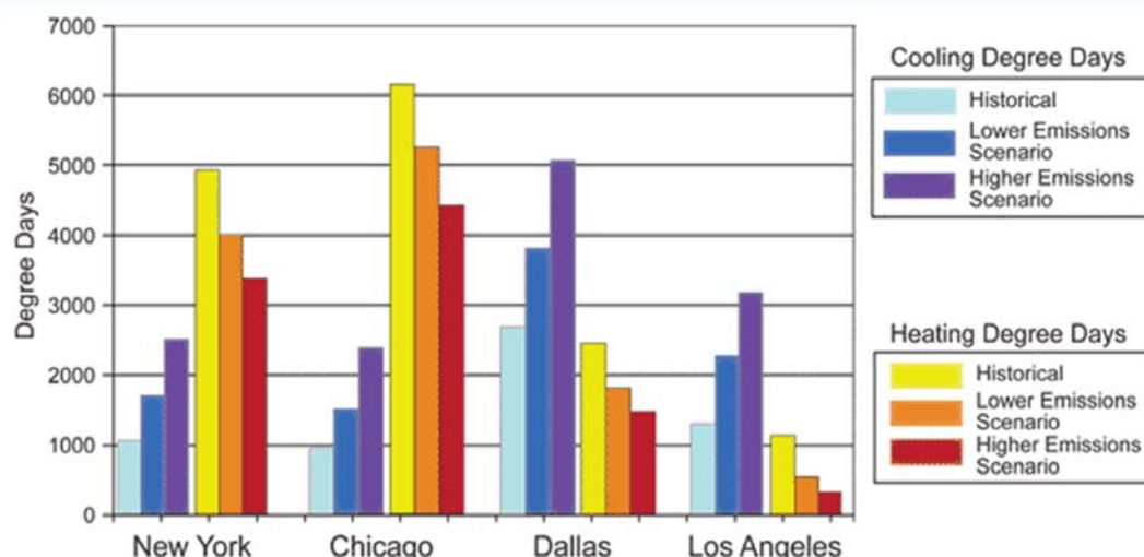
Figure 5. Changes in cooling degree days and heating degree days in the United States by 2080–2099, under a lower emissions scenario (B1) and a very high emissions scenario (A1FI)
