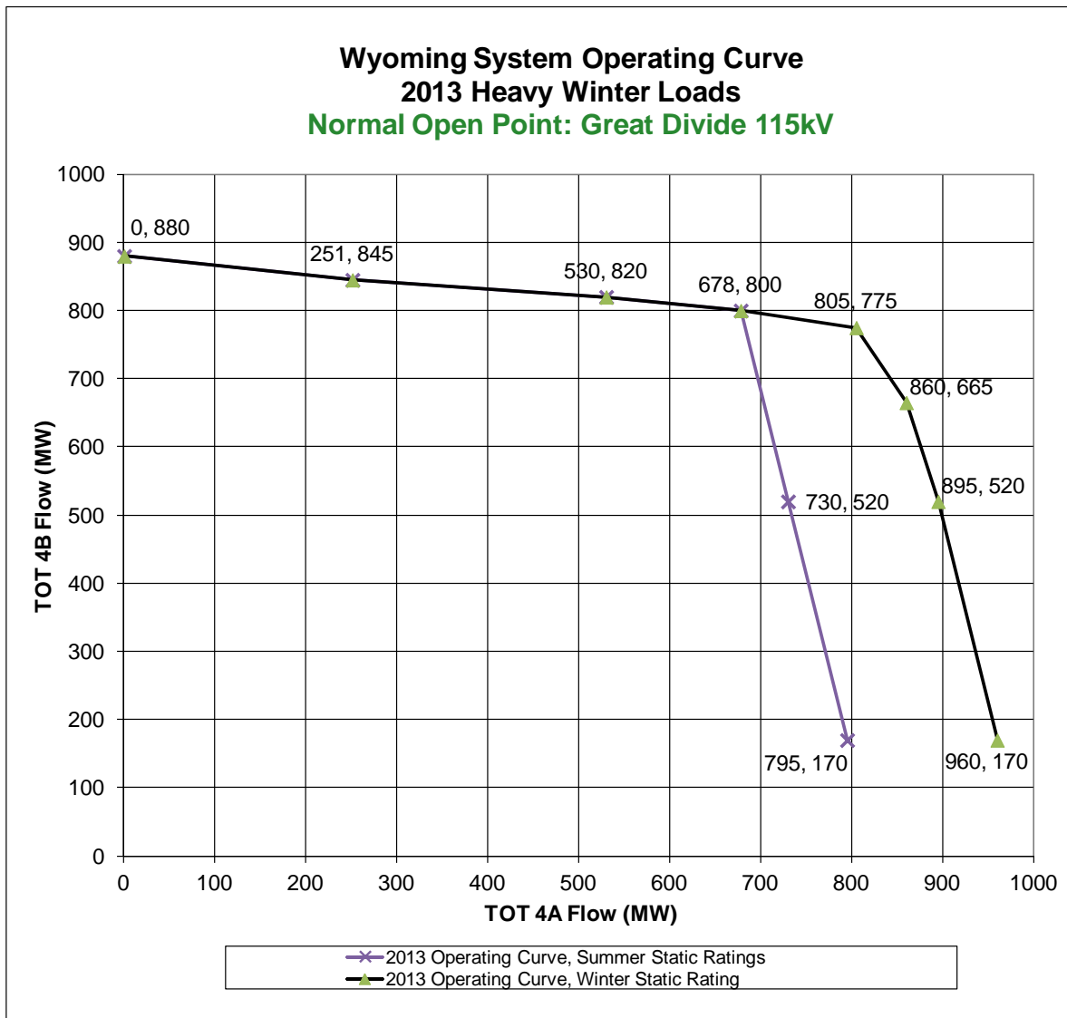
Figure 12 – TOT4A/TOT4B Nomogram
