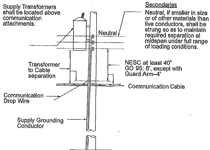
Figure 1 – Clearances Between Transformers and Communications Cables
