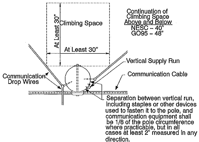
Figure 5—Climbing Space
