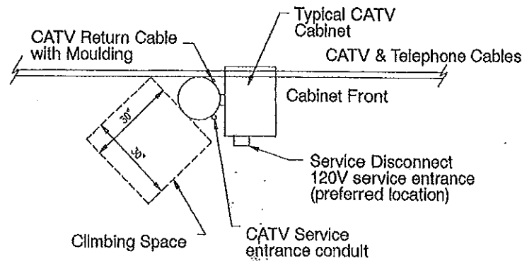
Figure 3 - Climbing Space
