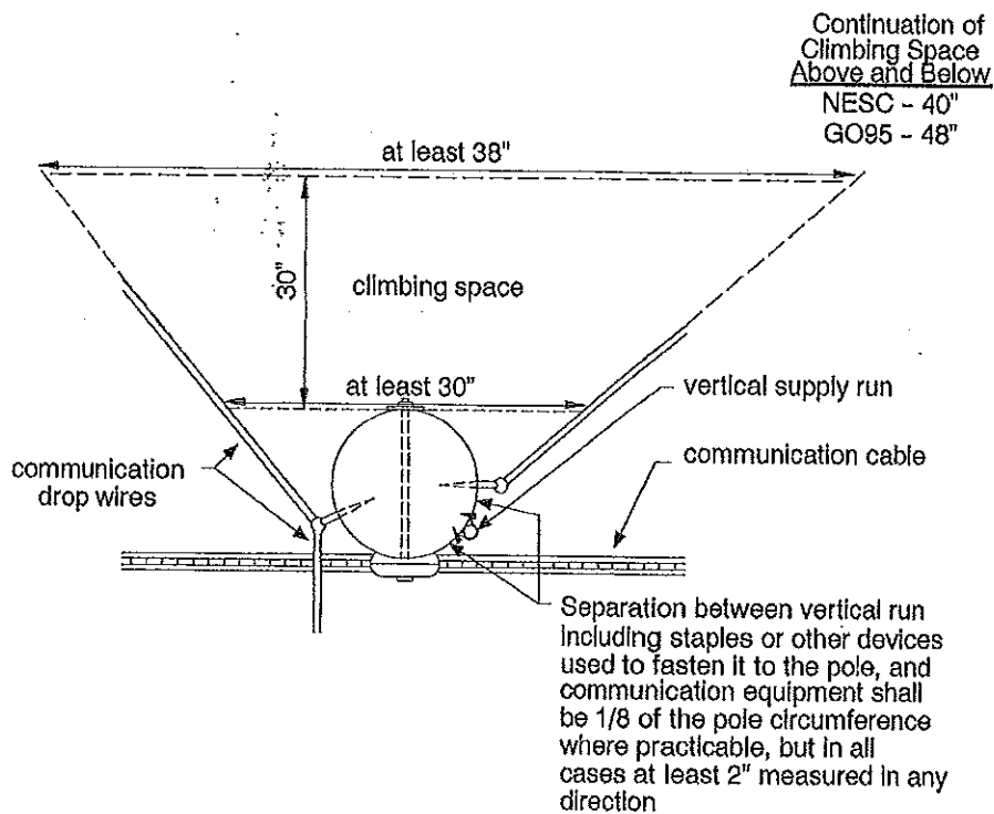
Figure 1 - Climbing Space
