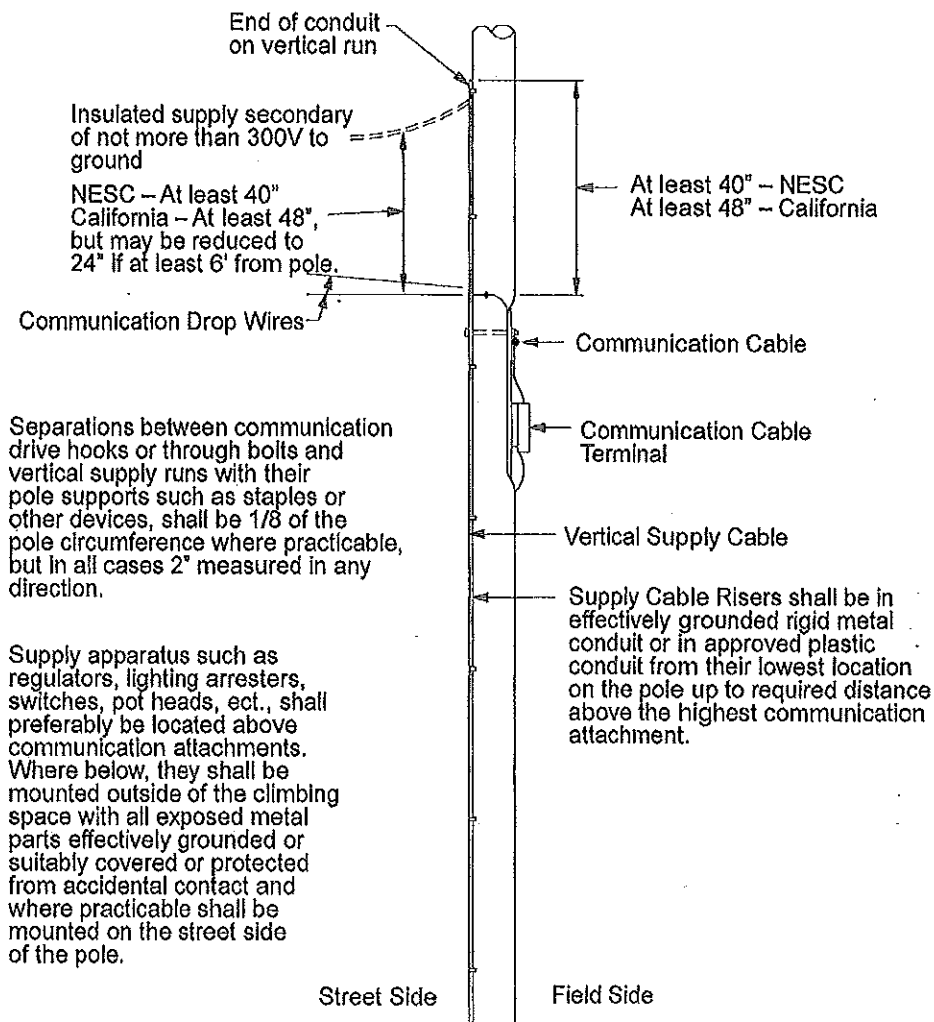
Figure 3 - Supply Riser on Joint Use Pole
