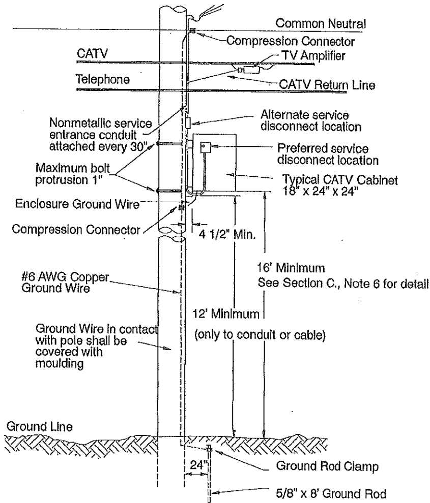
Figure 4 - Typical Installation of CATV Auxilliary Equipment with Grounding
