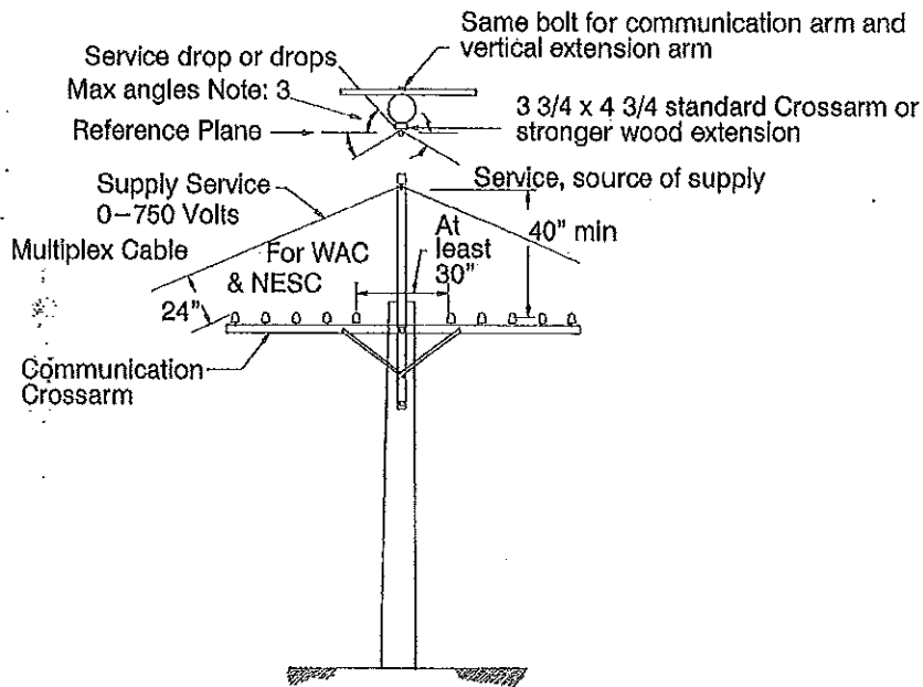
Figure 1 – Service Drop Contacts on Communications Poles
