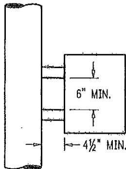
Figure 2 - Equipment Cabinet with Mounting Brackets
