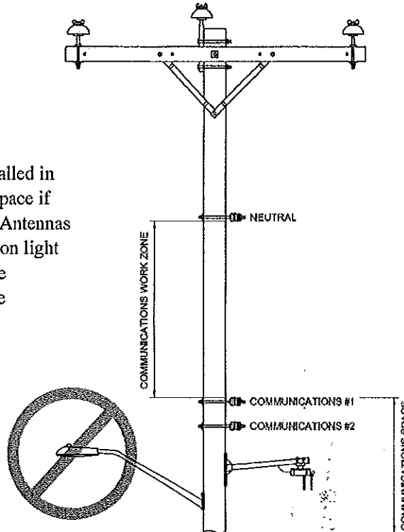
Figure 4—Antenna Installed on Pole in Communication Space
