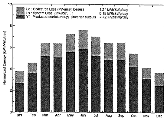
Normalized productions (per installed kWp): Nominal power 2527 kWp
