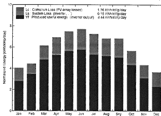
Normalized productions (per Installed kWp): Nominal power 3370 kWp
