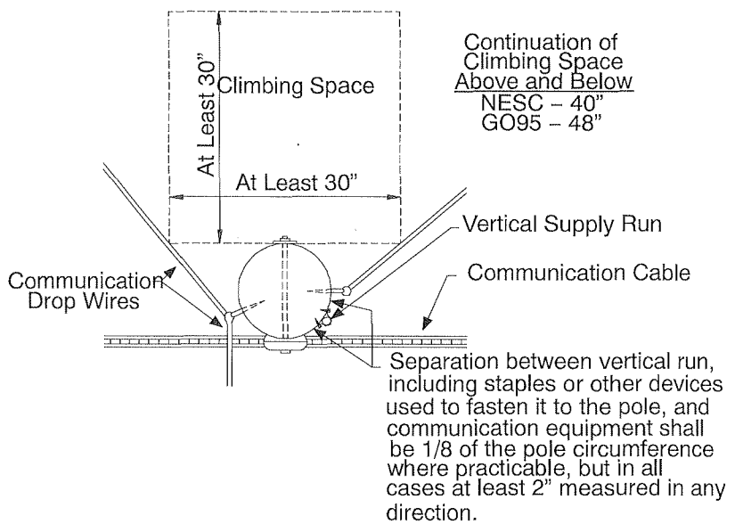
Figure 5—Climbing Space
