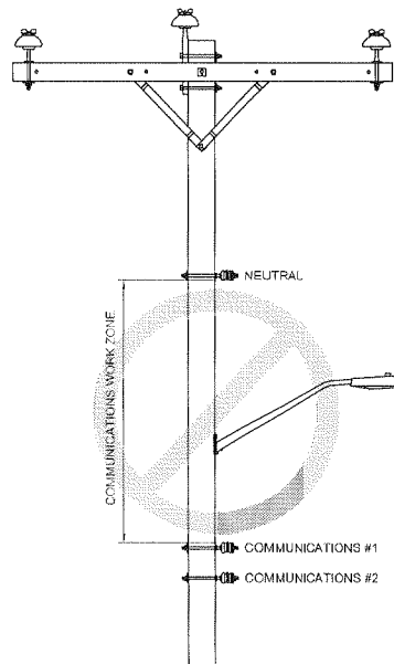
Figure 3—No Antennas on Streetlights in Communication Worker Safety Zone
