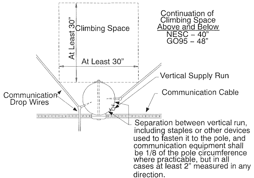
Figure 5—Climbing Space
