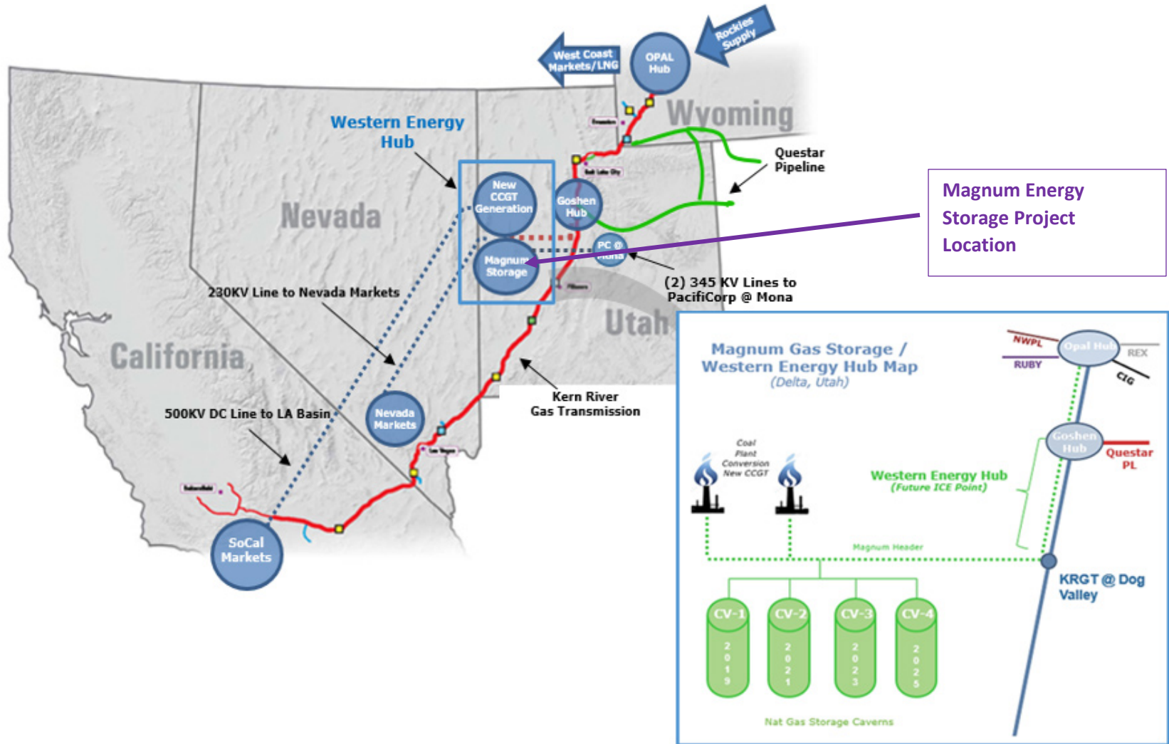
DPU Exhibit 2.8 Magnum Gas Storage Project, regional map and schematic
