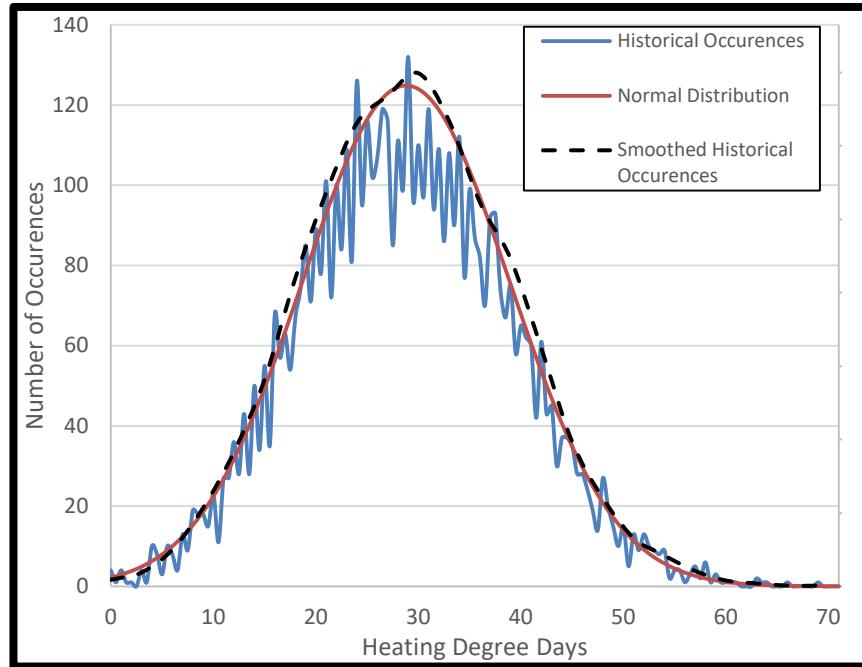
Figure 1: Winter Temperature Probability
