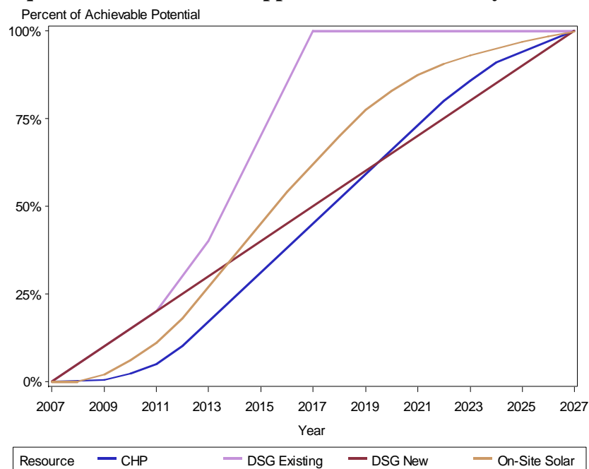
Figure 33. Acquisition Schedule for Supplemental Resources by Resource Category
