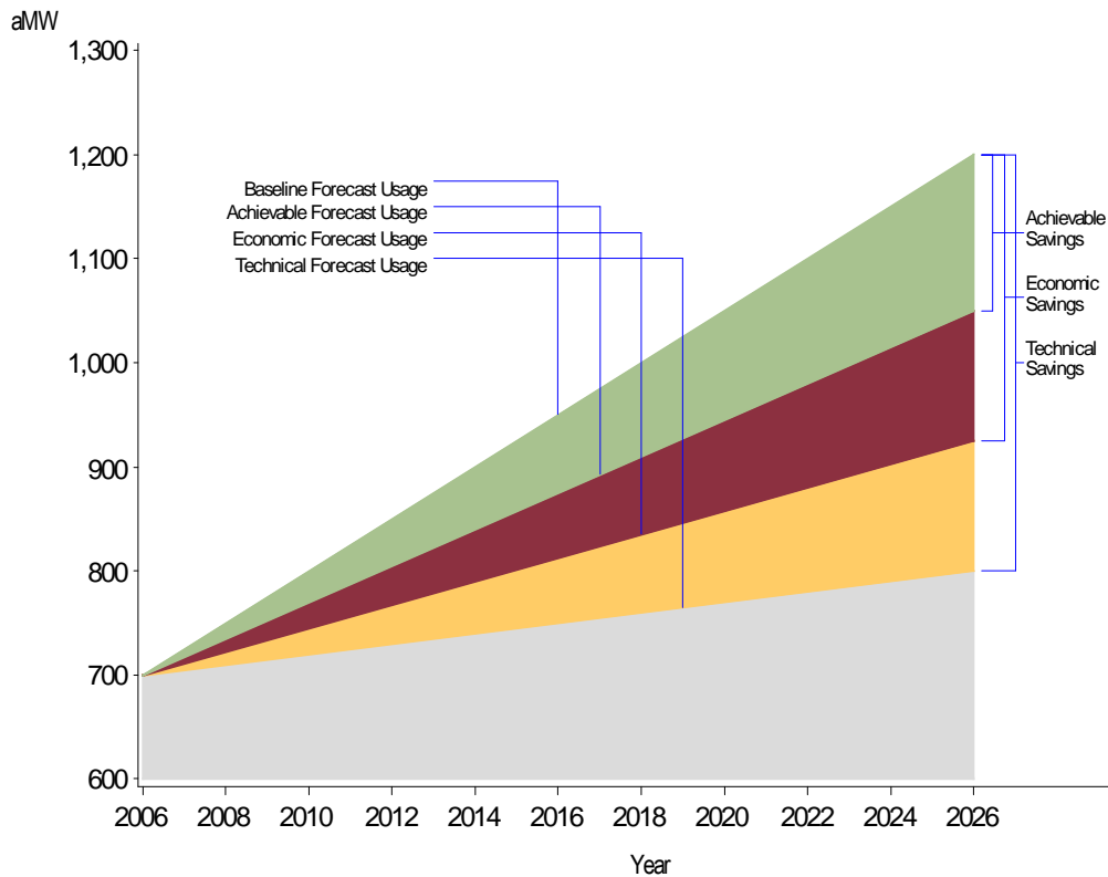
Figure 23. Representation of Alternative Forecast Approach to Estimation of Energy-Efficiency Potential
