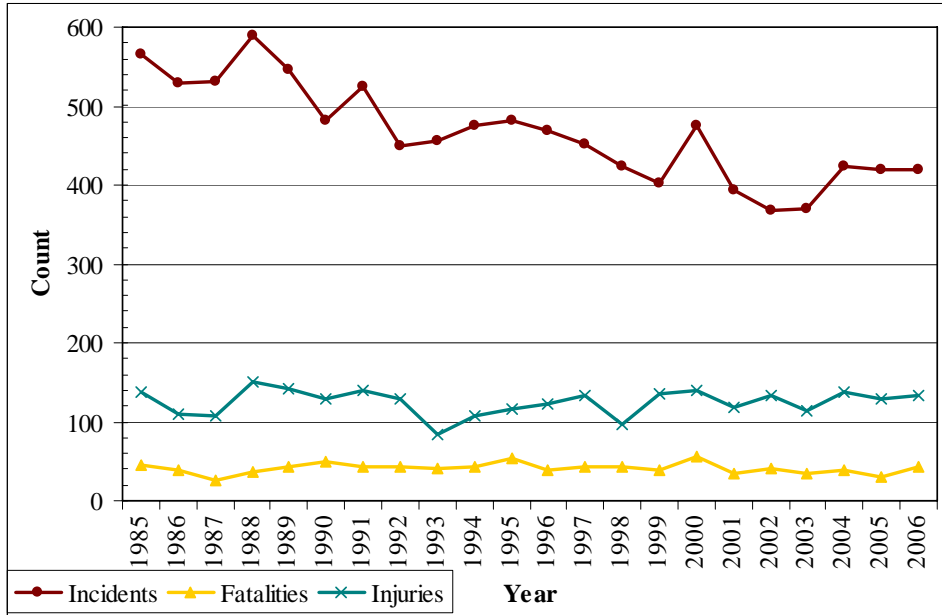
Figure 5. Annual Number of Incidents, Fatalities, and Injuries at Private Crossings, 1985–2006
