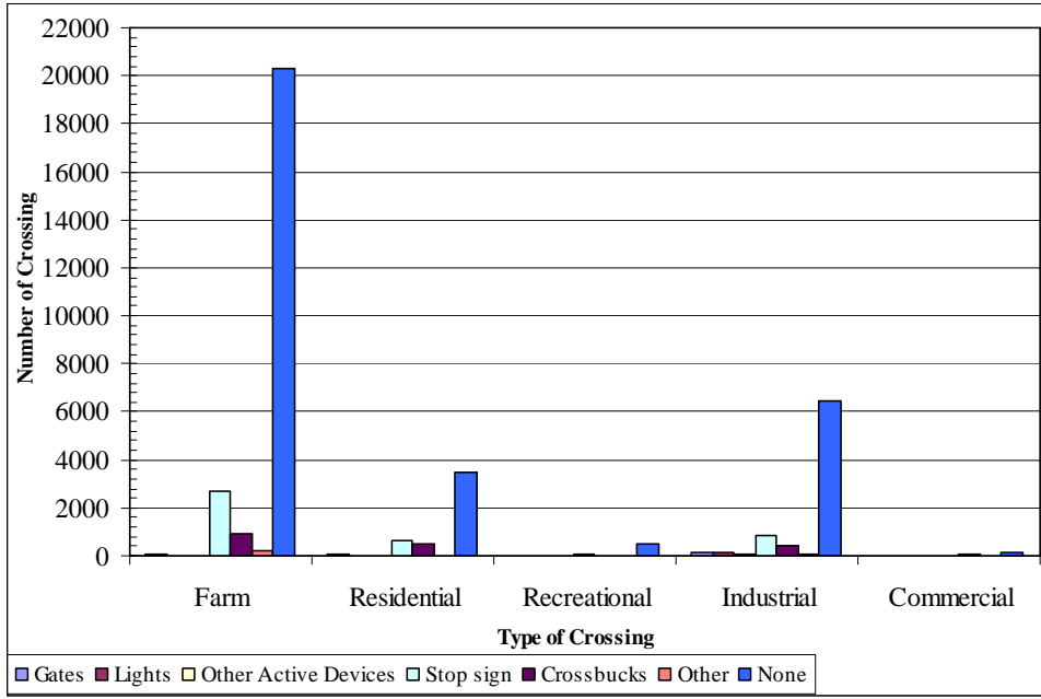
Figure 11. Number of Private Crossings Equipped with Warning Devices by Type of Crossing, November 2006
