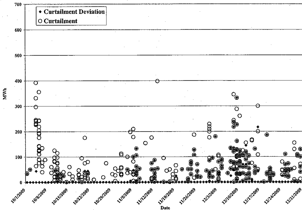
Figure 12: Curtailment and Curtailment Deviation Fourth Quarter of 2009
