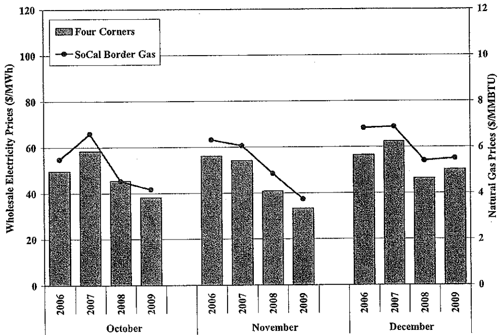
Figure 3: East Trends in Monthly Electricity and Natural Gas Prices Fourth Quarter, 2006–2009
