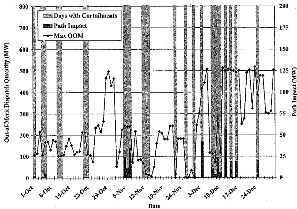
Figure 11: West Out-of-Merit Dispatch and Congestion Events Fourth Quarter of 2009
