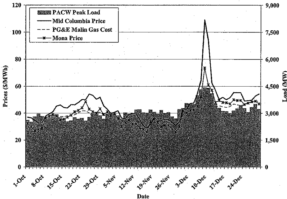
Figure 2: West Wholesale Prices and Peak Load, Fourth Quarter of 2009
