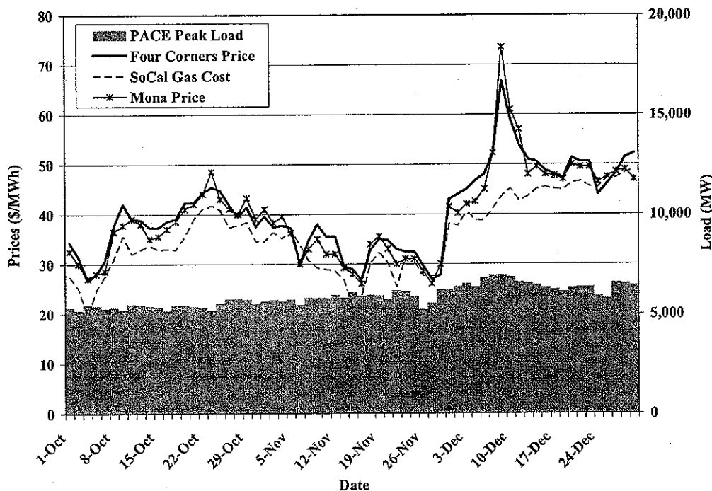
Figure 1: East Wholesale Prices and Peak Load, Fourth Quarter of 2009
