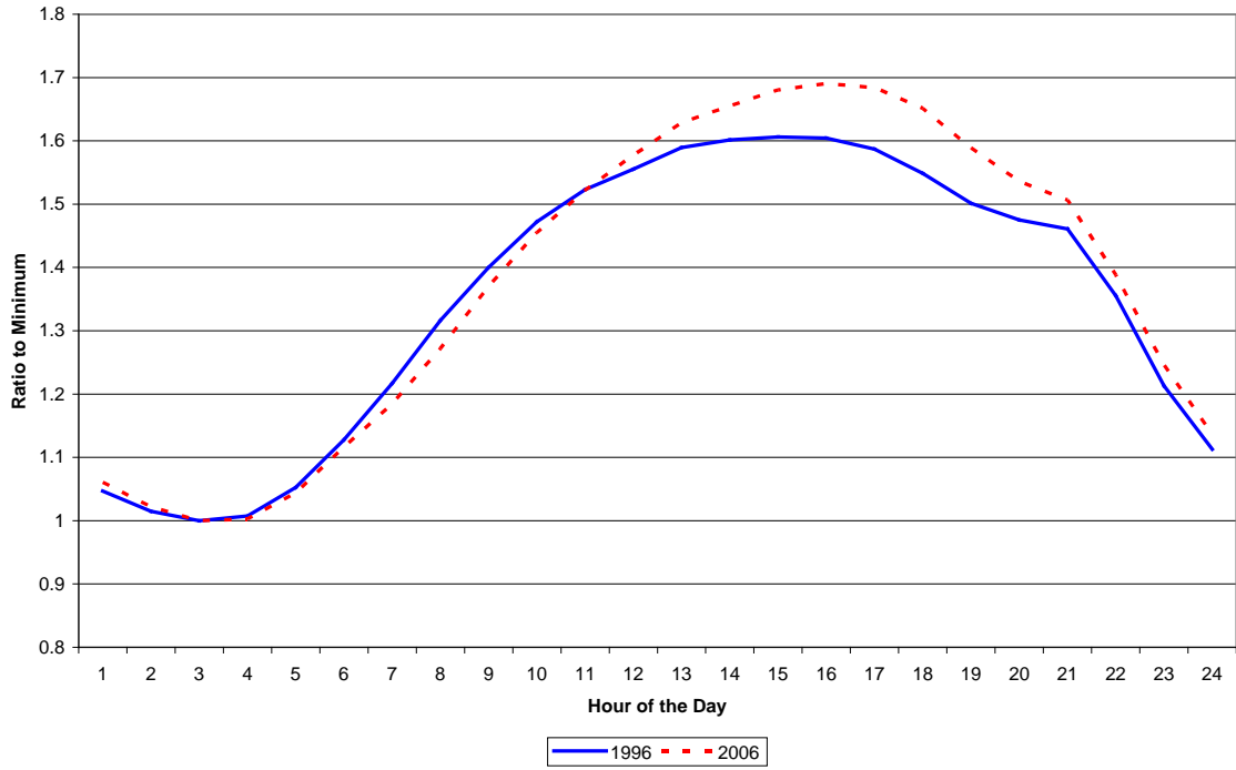
Average Summer Weekday Load Shapes-- Rocky Mountain Power (Utah)
