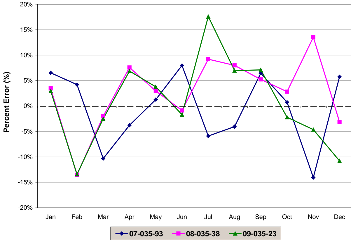
Figure 1: Accuracy of Energy Estimate from Load Research – Residential (Schedule 1)
