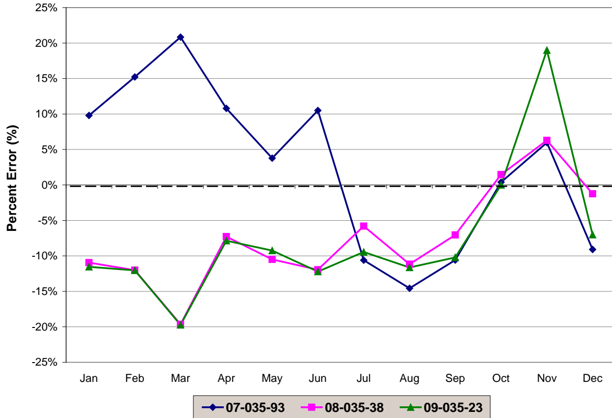
Figure 2: Accuracy of Energy Estimate from Load Research – Commercial (Schedule 6)
