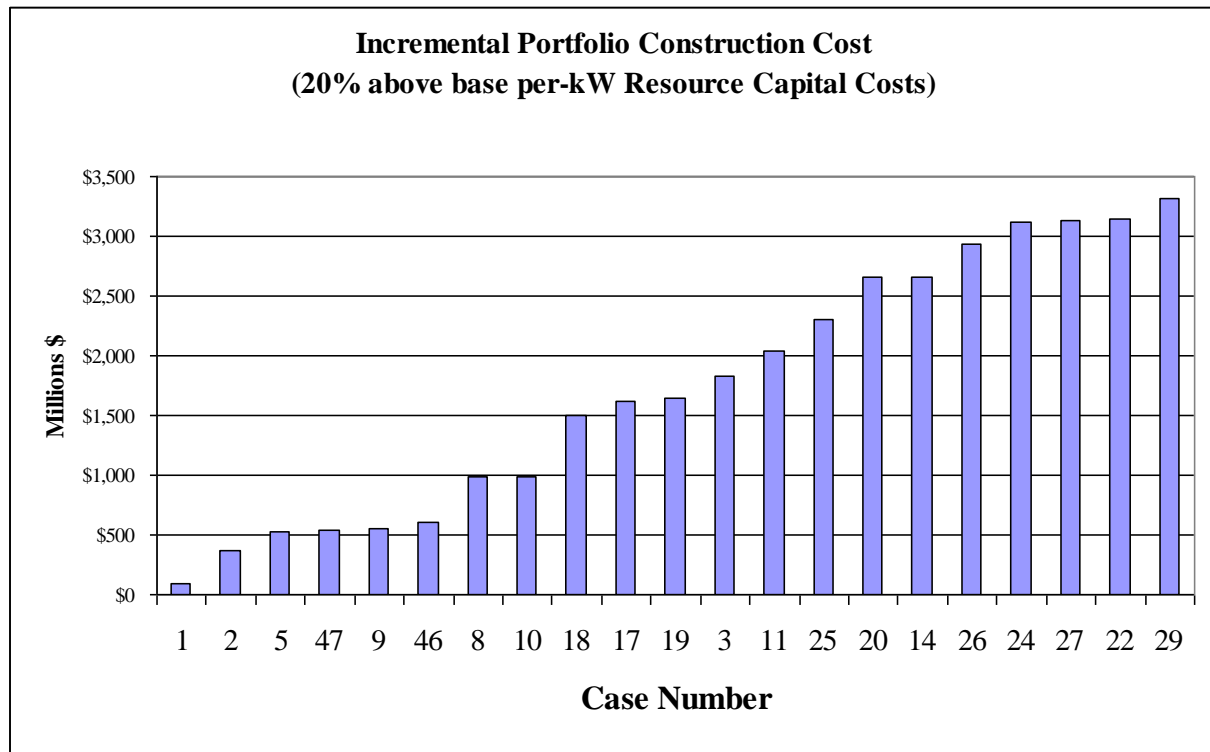
Figure 8.11 – Incremental Portfolio Capital Costs (20% increase from Base per-kW values)
