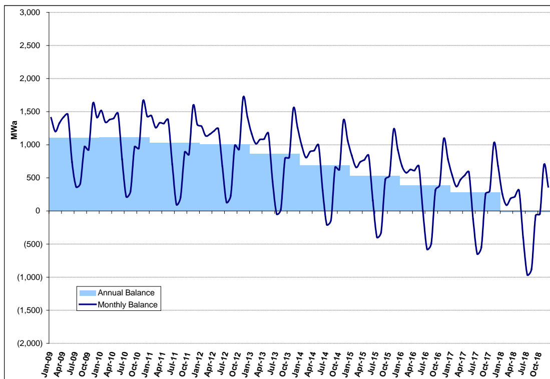
Figure 5.1208 – East Average Monthly and Annual Energy Balances
