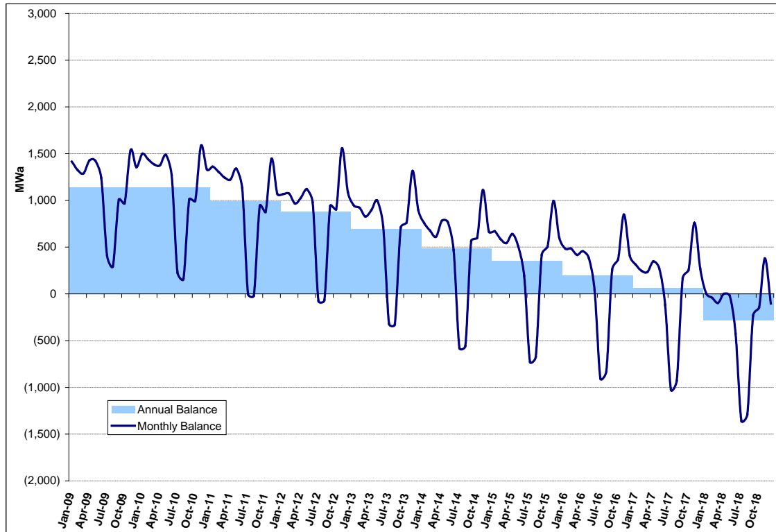
Figure 5.11 86 – System Average Monthly and Annual Energy Balances
