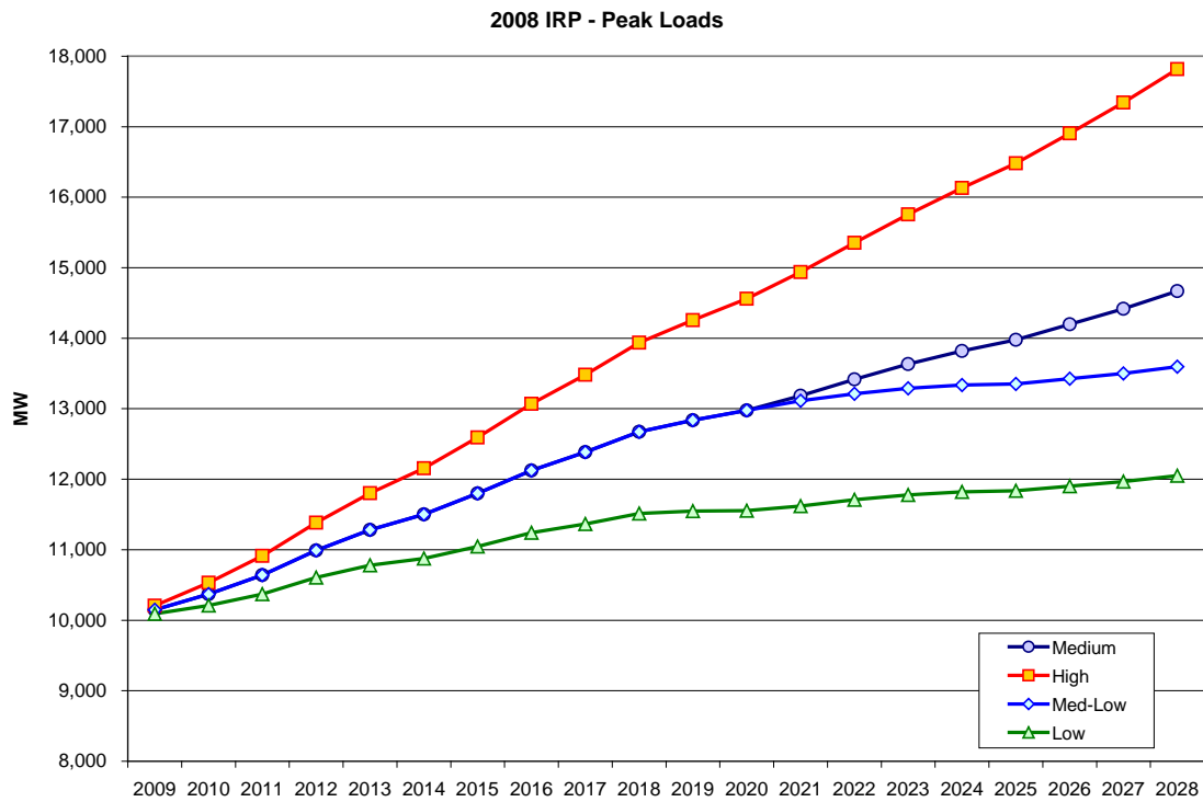
Figure 7.3 – Peak Load Growth Scenarios
