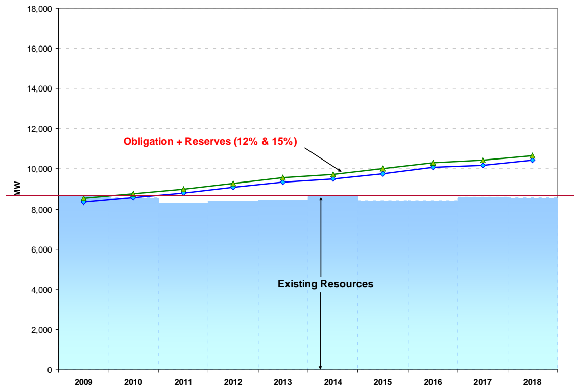
Figure 5.5—East Capacity Position Trend including Lake Side II
