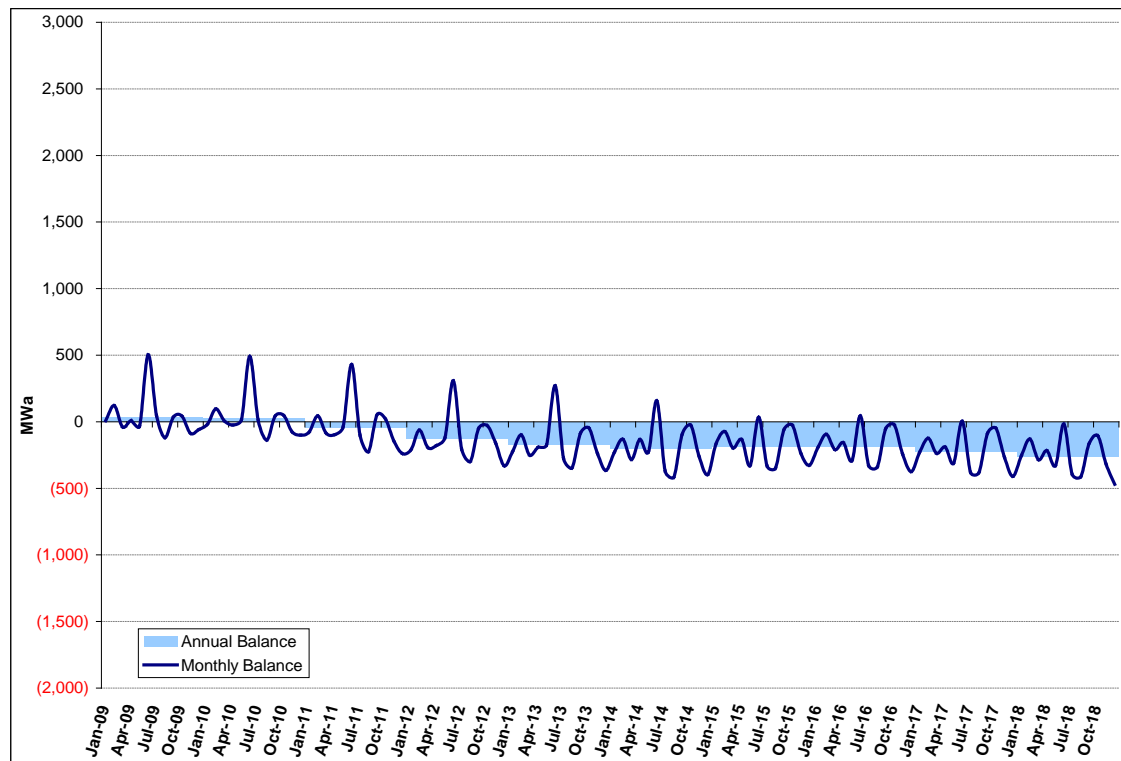
Figure 5.97 – West Average Monthly and Annual Energy Balances
