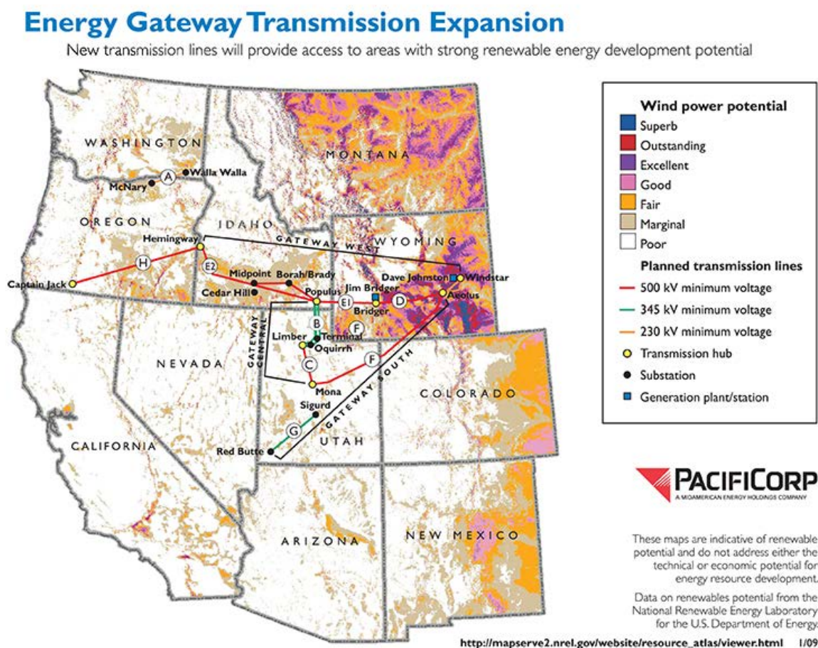
Figure 4.2 – Western States Wind Power Potential Up to 25,000 Megawatts
