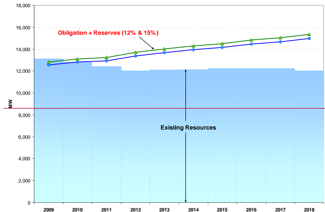
Figure 5.3 – System Capacity Position Trend including Lake Side II
