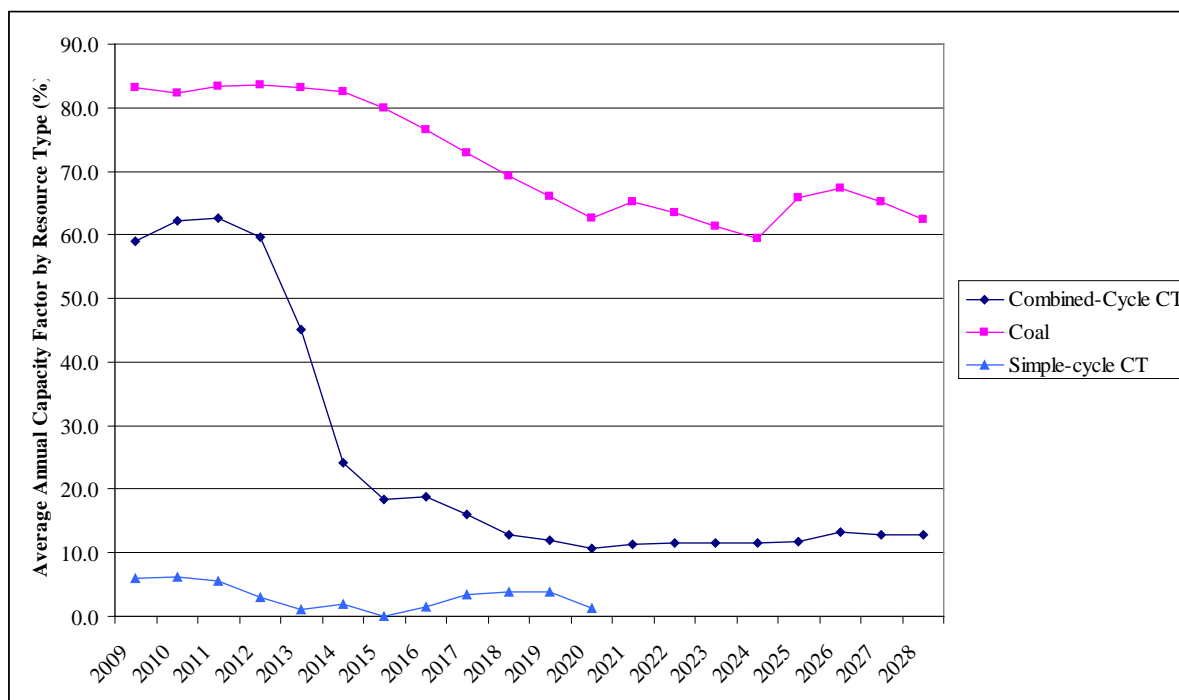
Figure 8.1 – Average Annual Capacity Factors by Resource Type, CO 2 Hard Cap Portfolio
