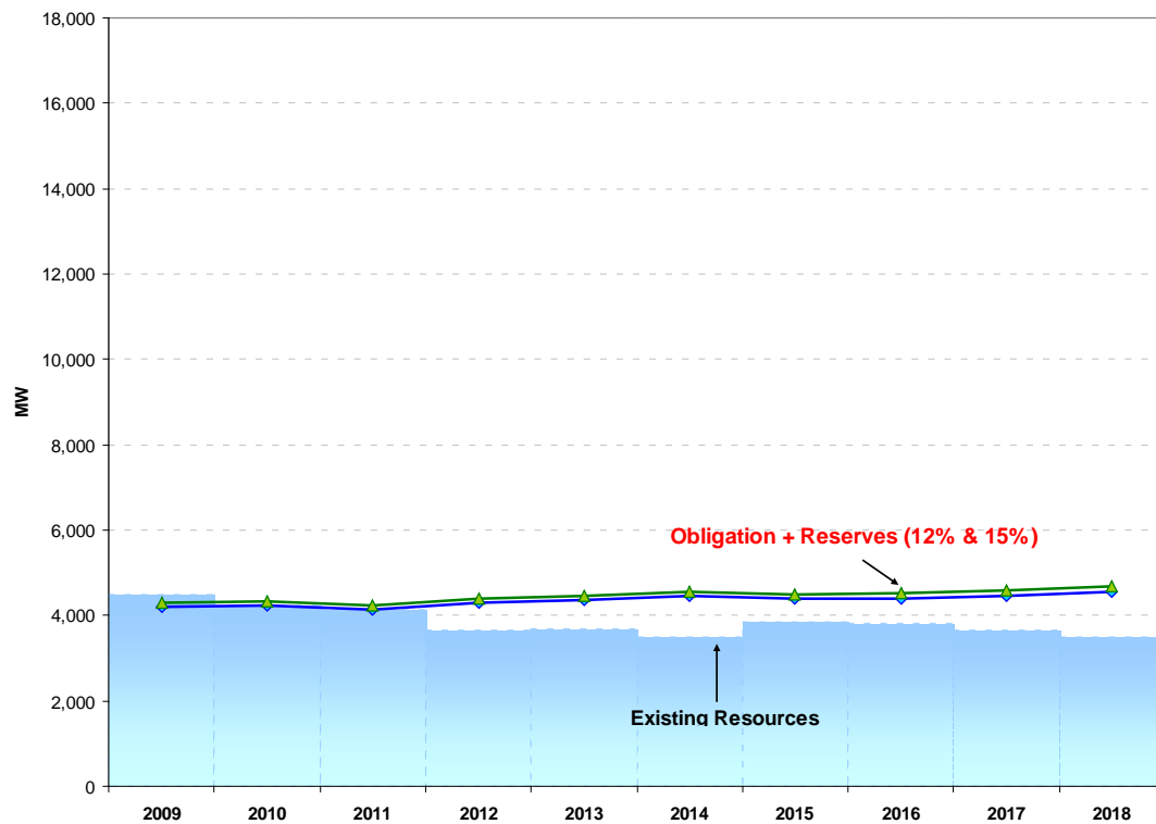
Figure 5.75 – East Capacity Position Trend without Lake Side II
