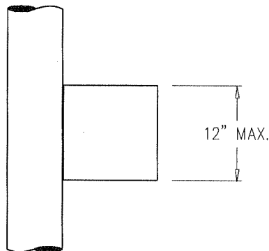
Figure 1 - Maximum Height of Directly Mounted Equipment Cabinet
