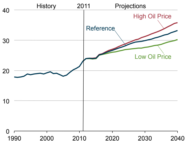
Figure 90. Total U.S. natural gas production in three oil price cases, 1990-2040 (trillion cubic feet per year)
