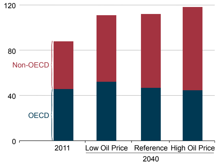
Figure 50. World petroleum and other liquids consumption by region in three cases, 2011 and 2040 (million barrels per day)
