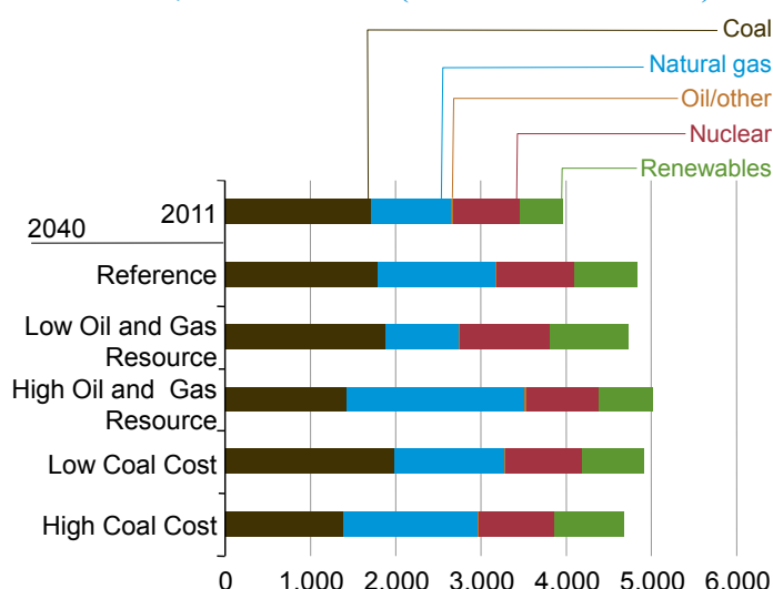
Figure 31. Power sector electricity generation by fuel in five cases, 2011 and 2040 (billion kilowatthours)
