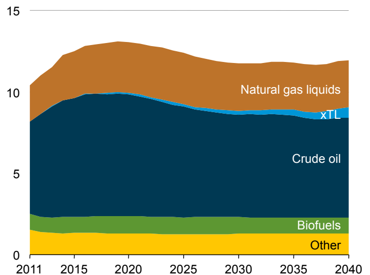
Figure 94. U.S. production of petroleum and other liquids by source, 2011-2040 (million barrels per day)
