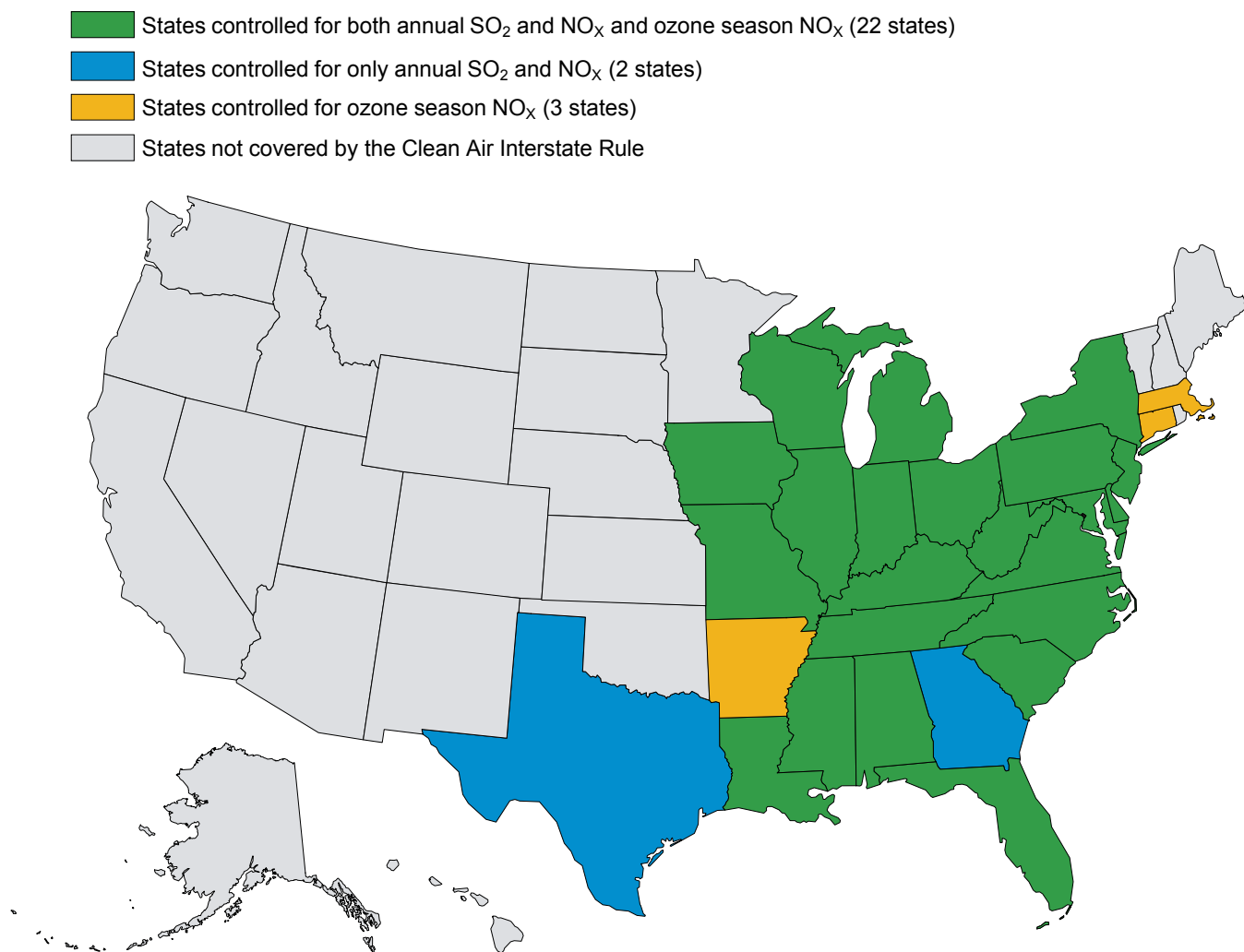
Figure 11. States covered by CAIR limits on emissions of sulfur dioxide and nitrogen oxides
