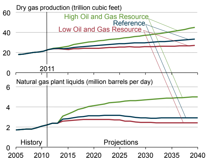
Figure 42. U.S. production of dry natural gas and natural gas plant liquids in three cases, 2005-2040
