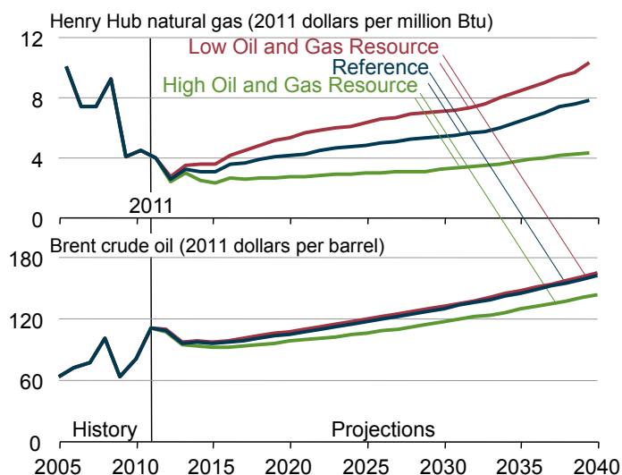
Figure 41. U.S. Brent crude oil and Henry Hub natural gas spot market prices in three cases, 2005-2040
