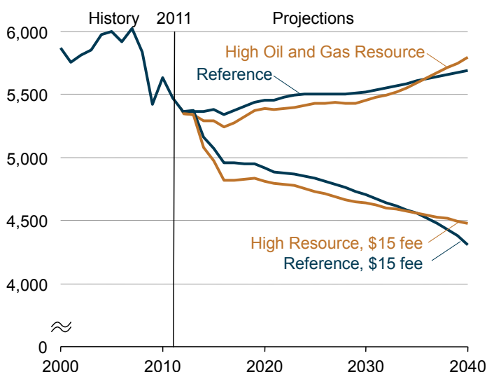
Figure 5. Energy-related carbon dioxide emissions in four cases, 2000-2040 (million metric tons)
