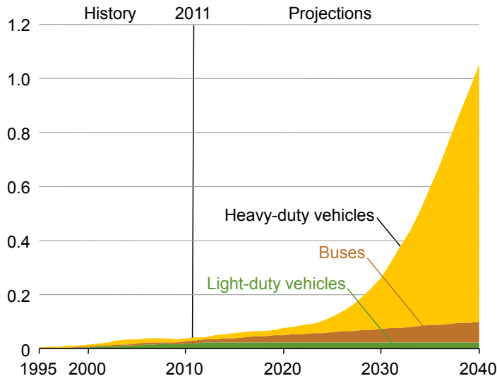
Figure 74. Natural gas consumption in the transportation sector, 1995-2040 (quadrillion Btu)
