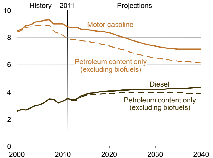
Figure 102. U.S. motor gasoline and diesel fuel consumption, 2000-2040 (million barrels per day)
