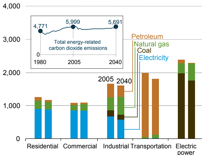
Figure 108. U.S. energy-related carbon dioxide emissions by sector and fuel, 2005 and 2040 (million metric tons)
