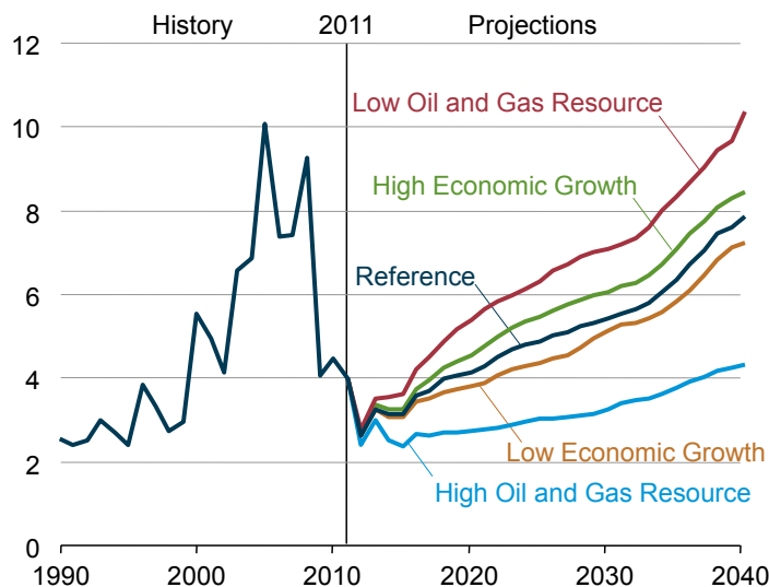
Figure 88. Annual average Henry Hub spot prices for natural gas in five cases, 1990-2040 (2011 dollars per million Btu)
