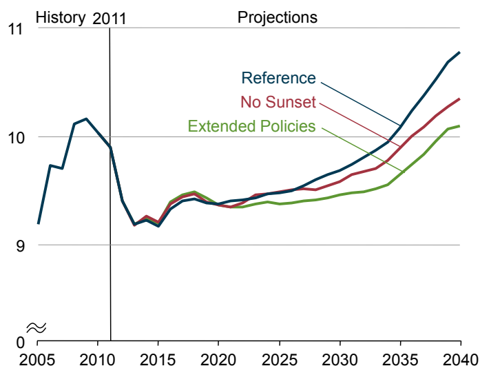
Figure 20. Average electricity prices in three cases, 2005-2040 (2011 cents per kilowatthour)
