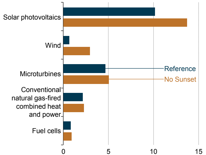
Figure 62. Additions to electricity generation capacity in the commercial sector in two cases, 2011-2040 (gigawatts)
