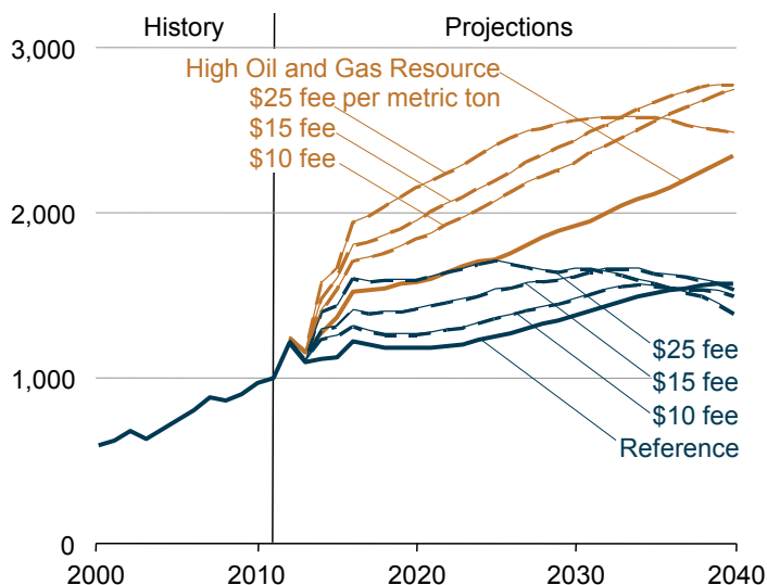
Figure 112. Natural gas-fired electricity generation in six CO 2 fee cases, 2000-2040 (billion kilowatthours)
