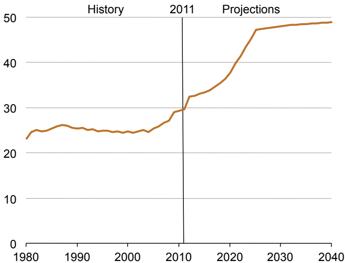
Figure 71. Average fuel economy of new light-duty vehicles, 1980-2040 (miles per gallon, CAFE compliance values)
