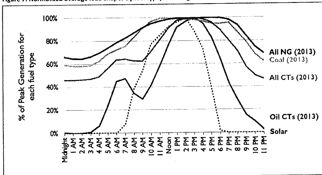
Figure 7: Normalized average load shapes by fuel type, including estimated shape of solar
