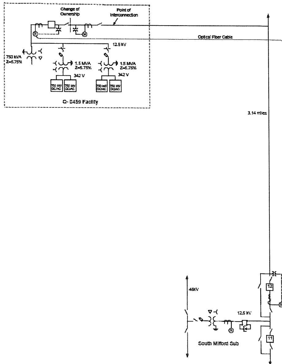
Figure 1: Generation One Line Diagram
