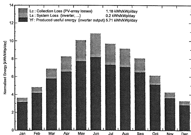
Normalized productions (per installed kWp): Nominal power 3900 kWp
