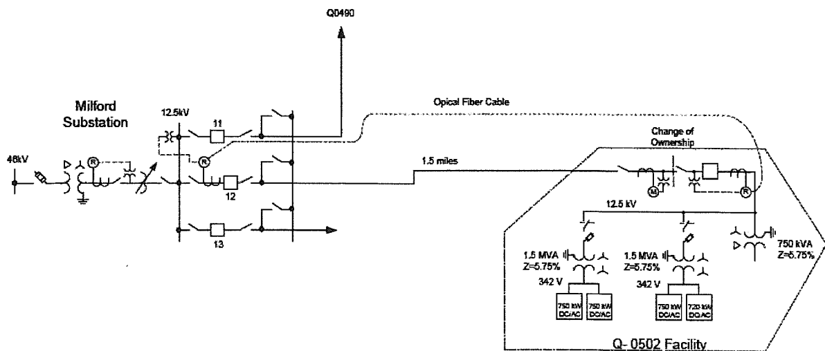
Figure 3: System One Line Diagram
