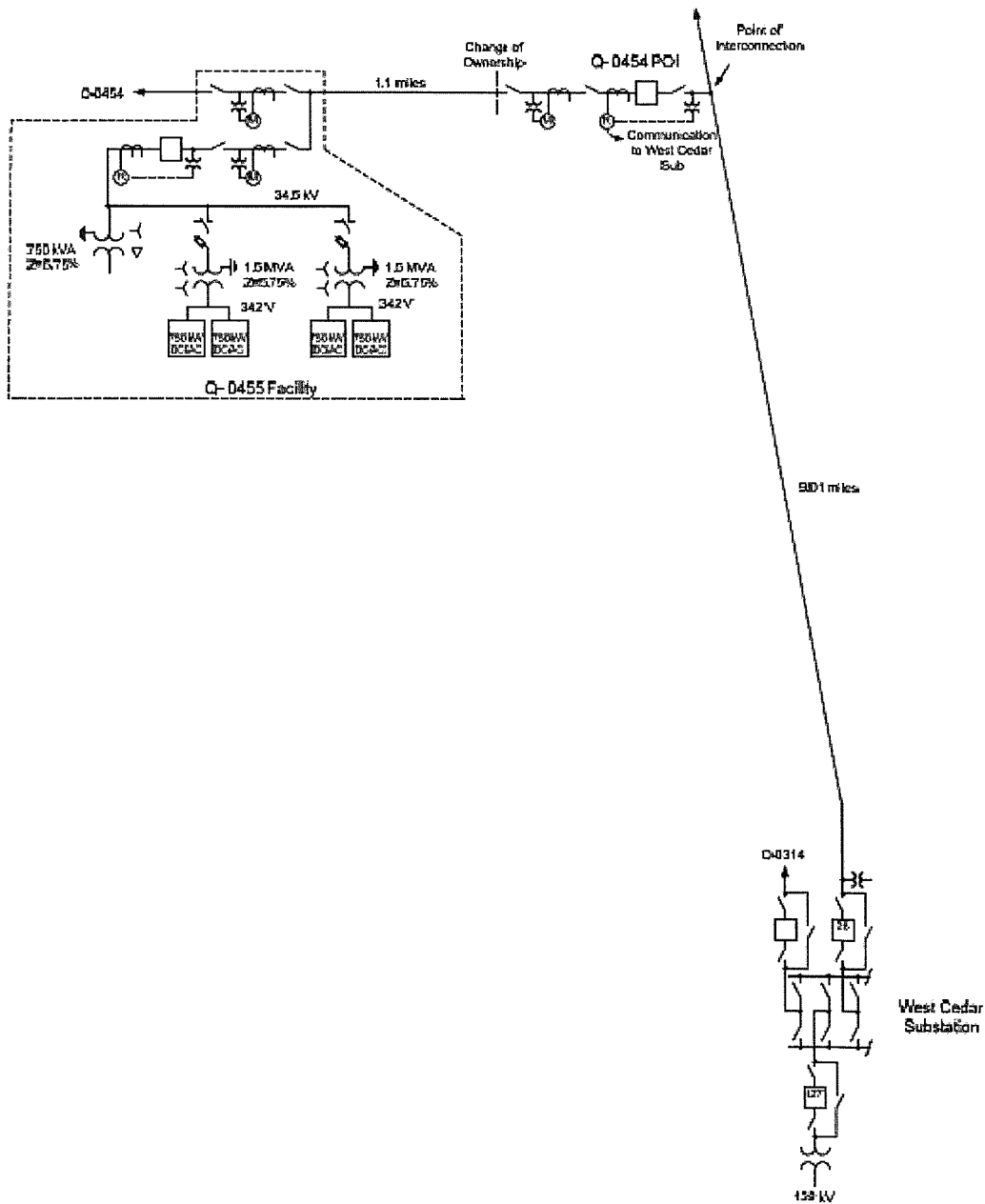
Figure 1: System One Line Diagram
