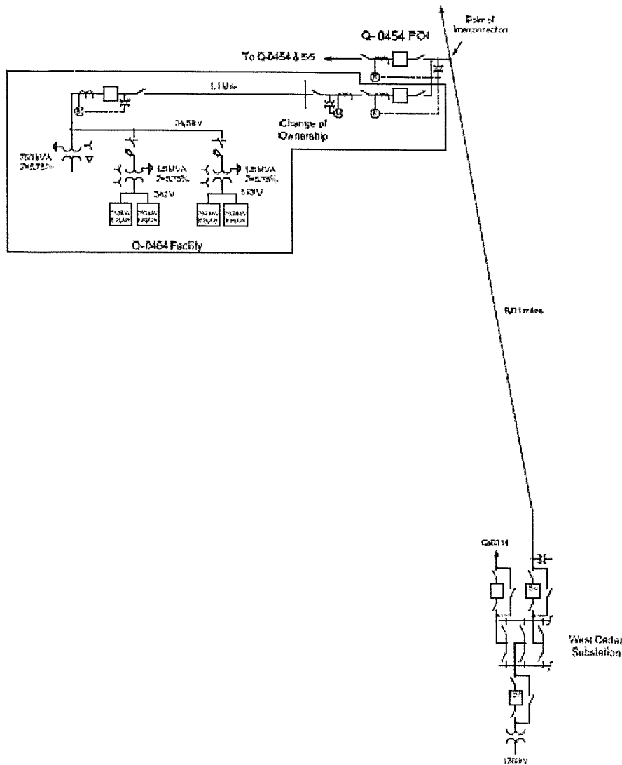
Figure 1: System One Line Diagram
