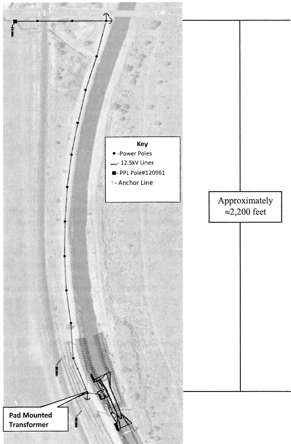
Figure 3 Proposed Monroe Drop Transmission Route
