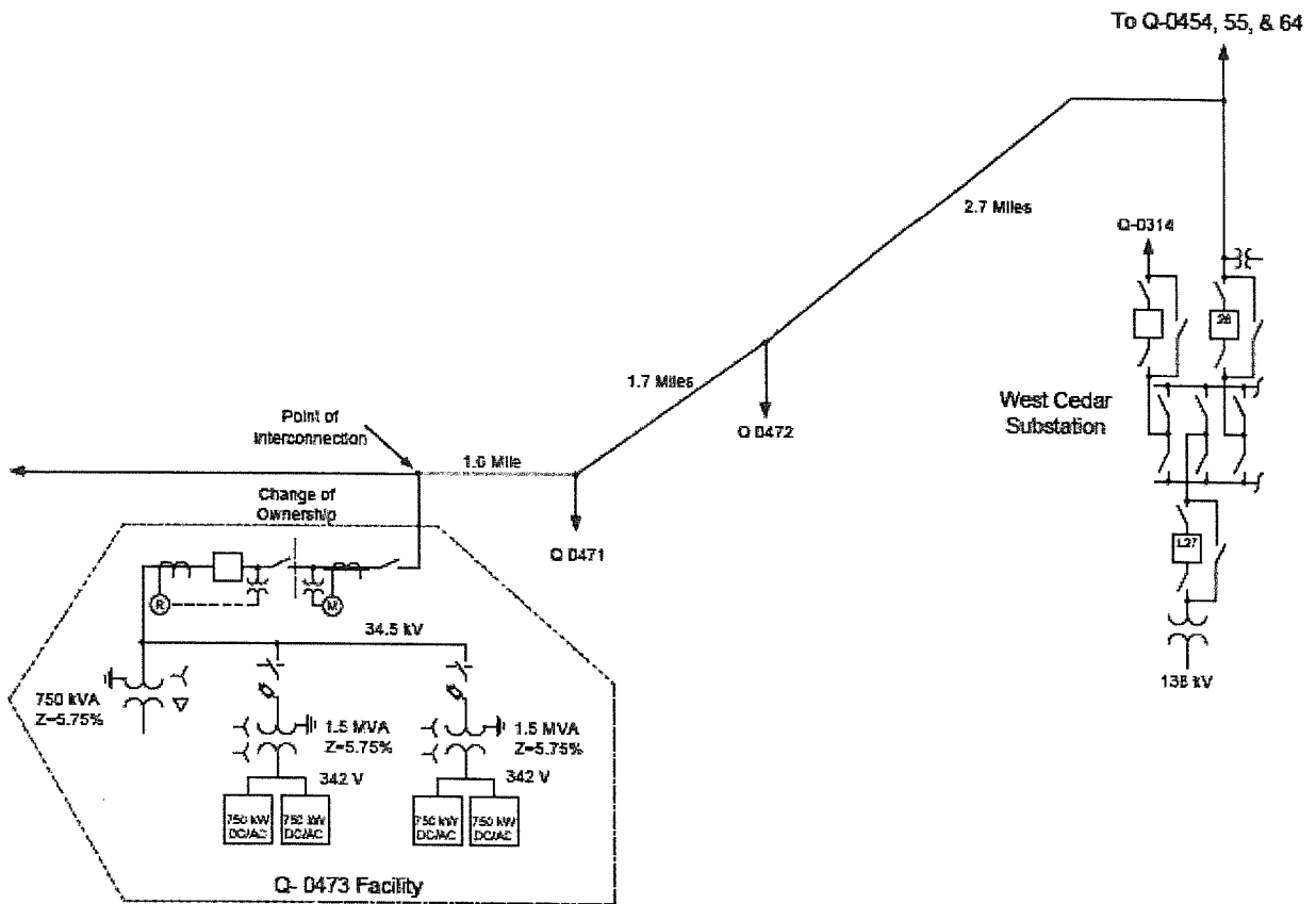
Figure 1: System One Line Diagram
