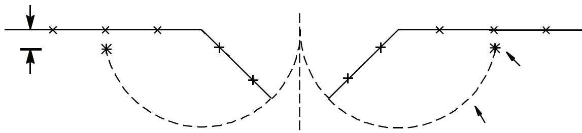
Figure 1—Inward Gate Swing
