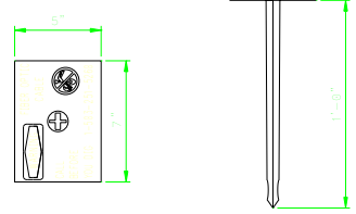
DETAIL E – GROUND MARKER
