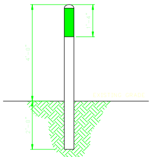
DETAIL D – FIBER ROUTE MARKER POST
