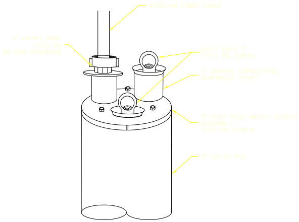
DETAIL C – 3" DUCT PLUG ASSEMBLY
