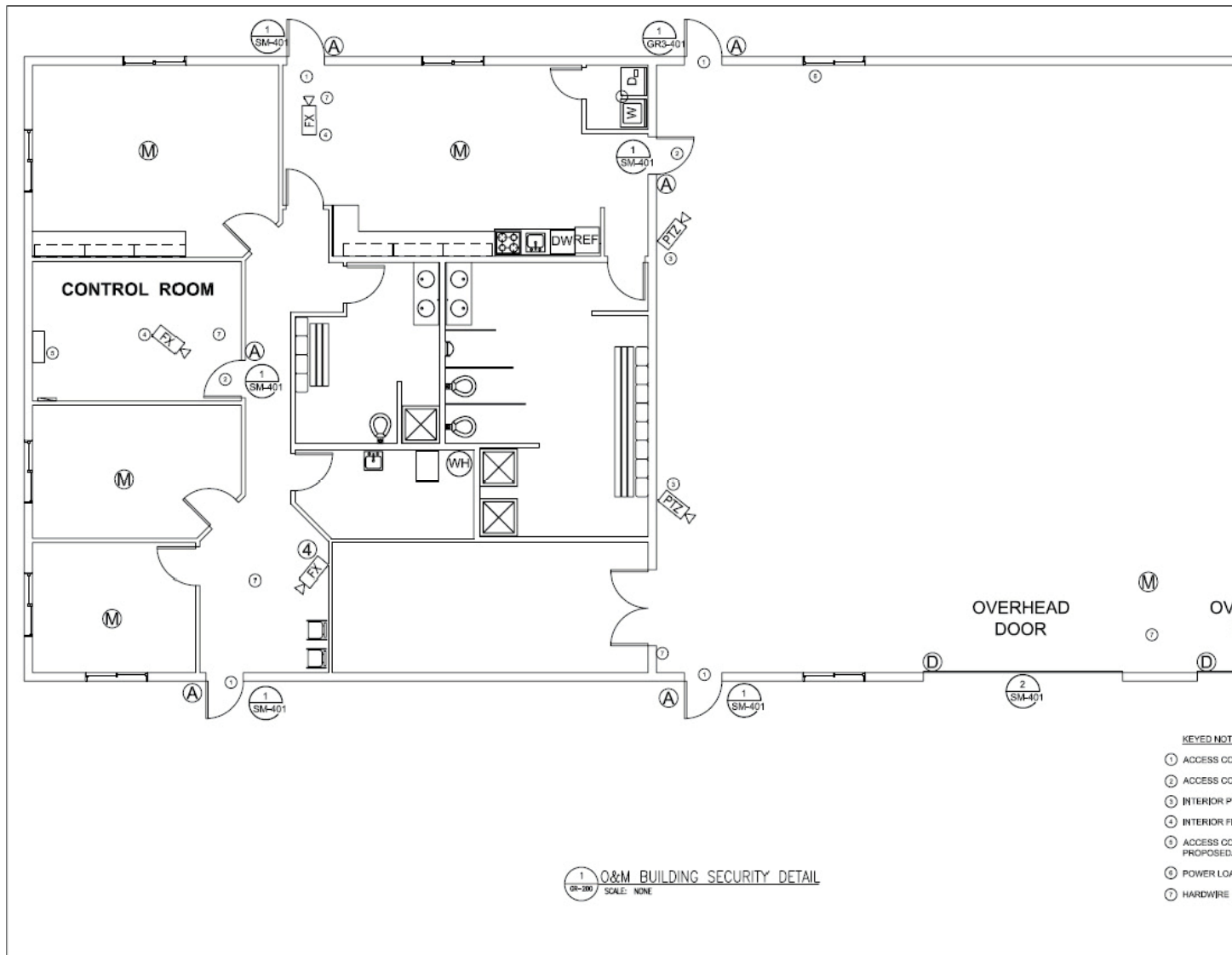
Figure 1: Indicative Operations and Maintenance Building Layout for projects up to 150 MW
