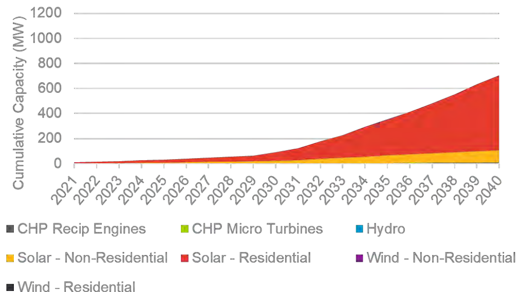
Figure 21. Cumulative Capacity Installations by Technology (MW AC), Oregon Base Case
