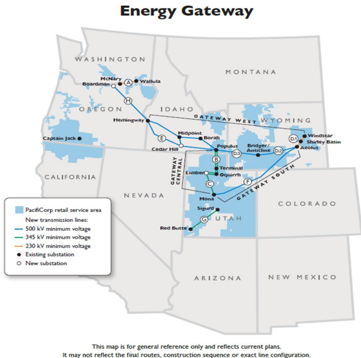
Figure 3.1 – Energy Gateway Map
