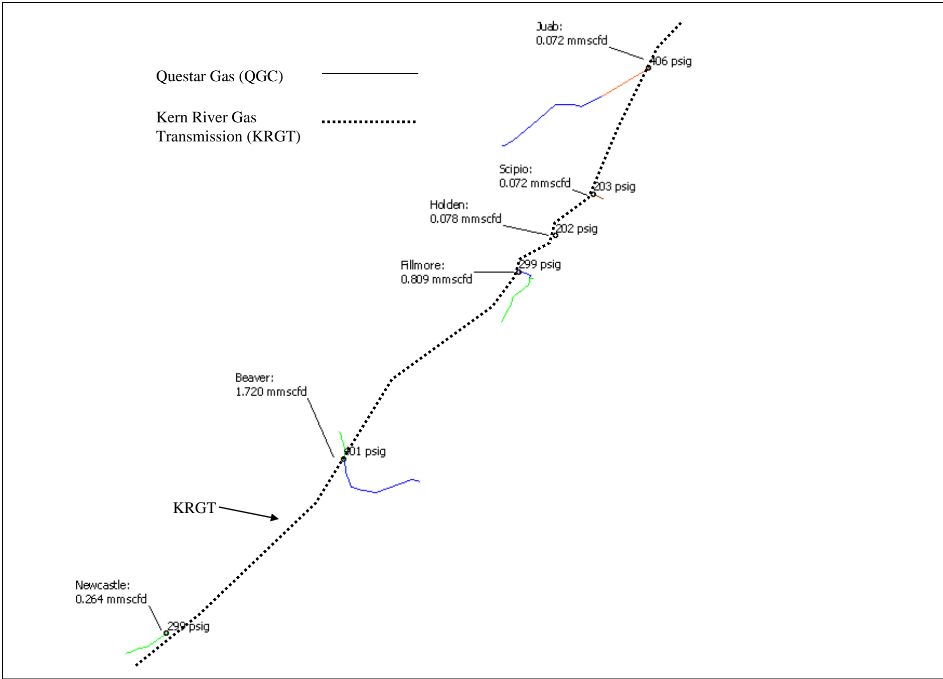
Exhibit 4.2 – Central System - Typical Winter Day
