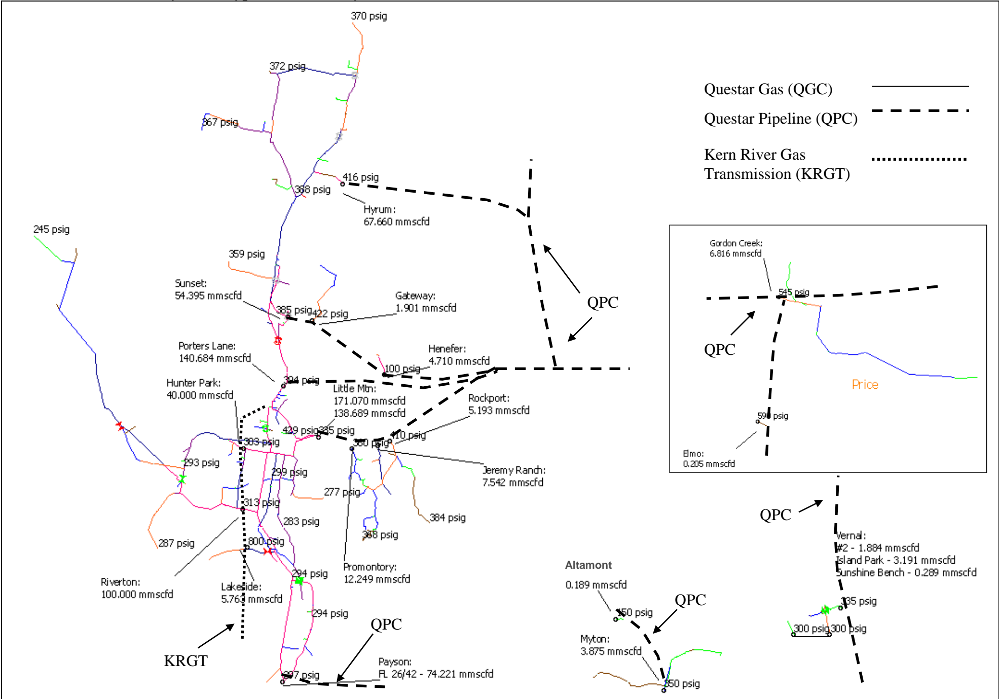
Exhibit 4.1 – Northern System –Typical Winter Day
