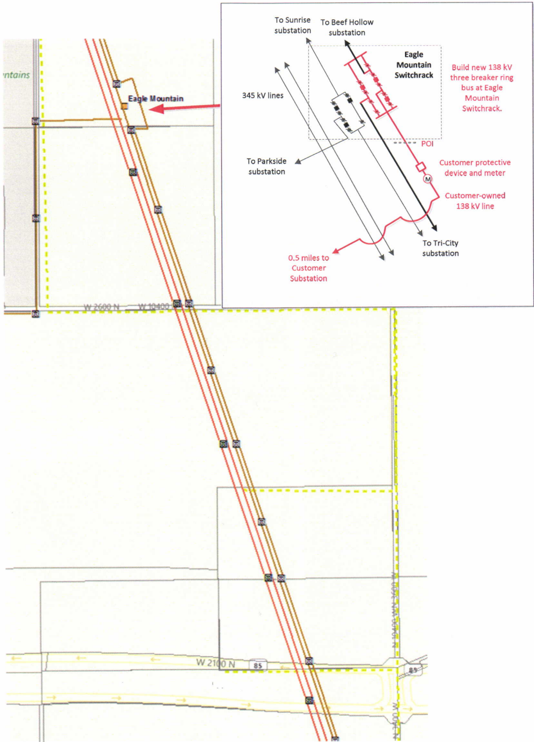
Diagram of the existing transmission system and after the connection of the Customer's Project
