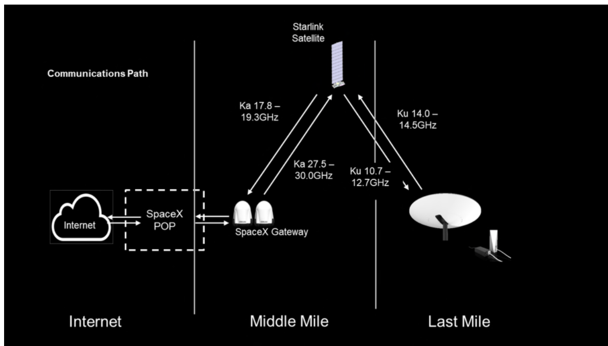
112 Figure 1 – Starlink Network Architecture
